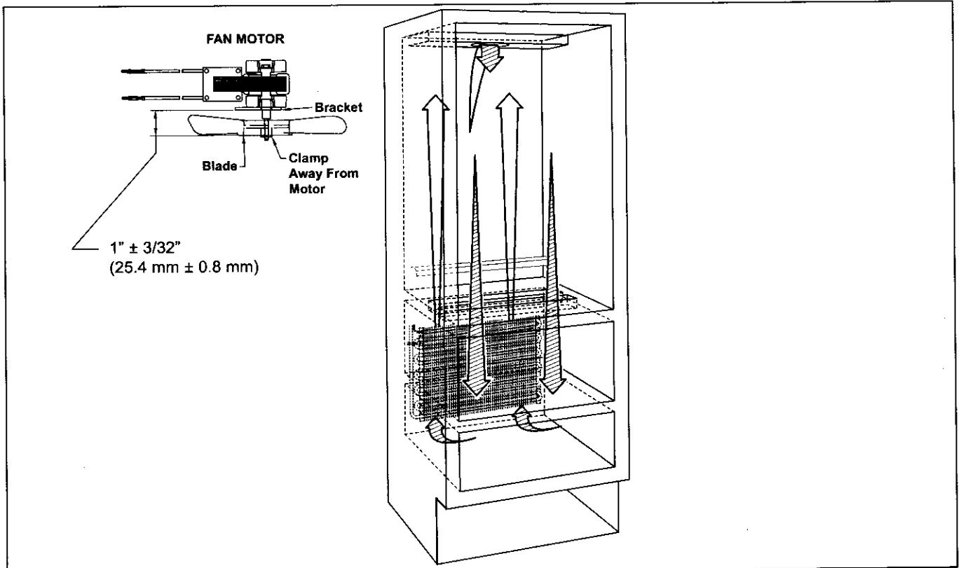
Figure 5-3. 700TF/I-3 Air Flow and Fan Blade Spacing
