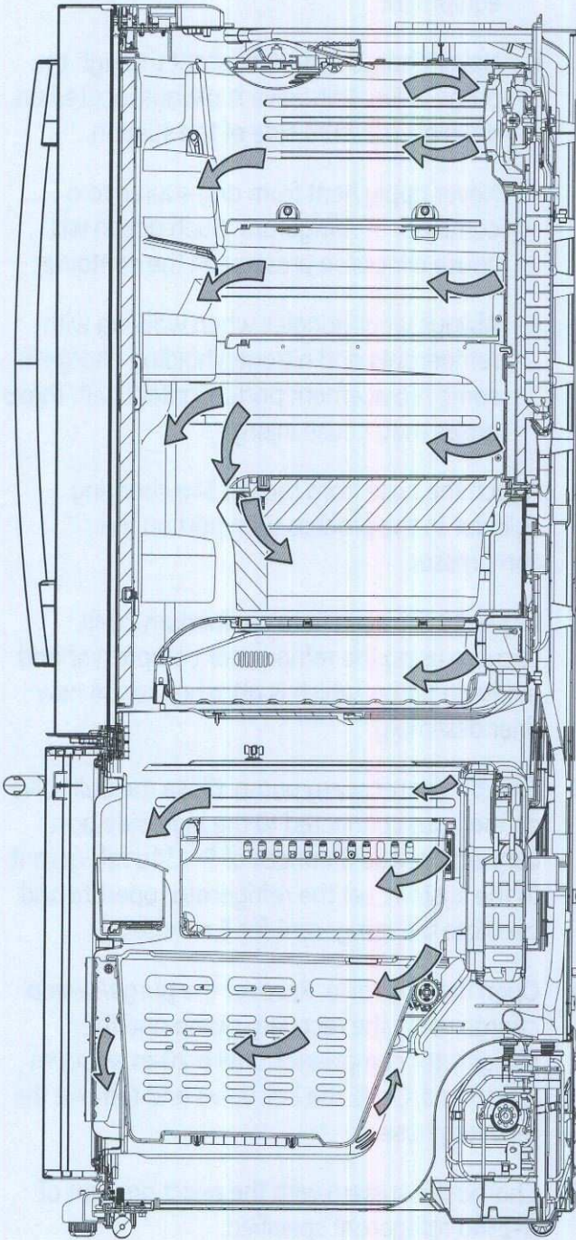
Air Flow (side view)
