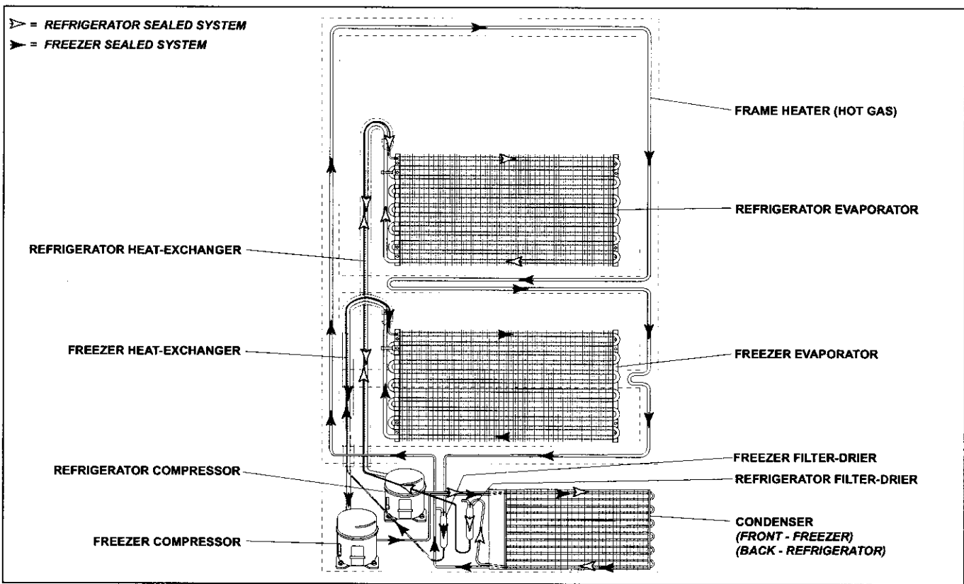
Figure 4-7. Models 700TC/I-3 and 736TC/I-3 Refrigerant Flow
