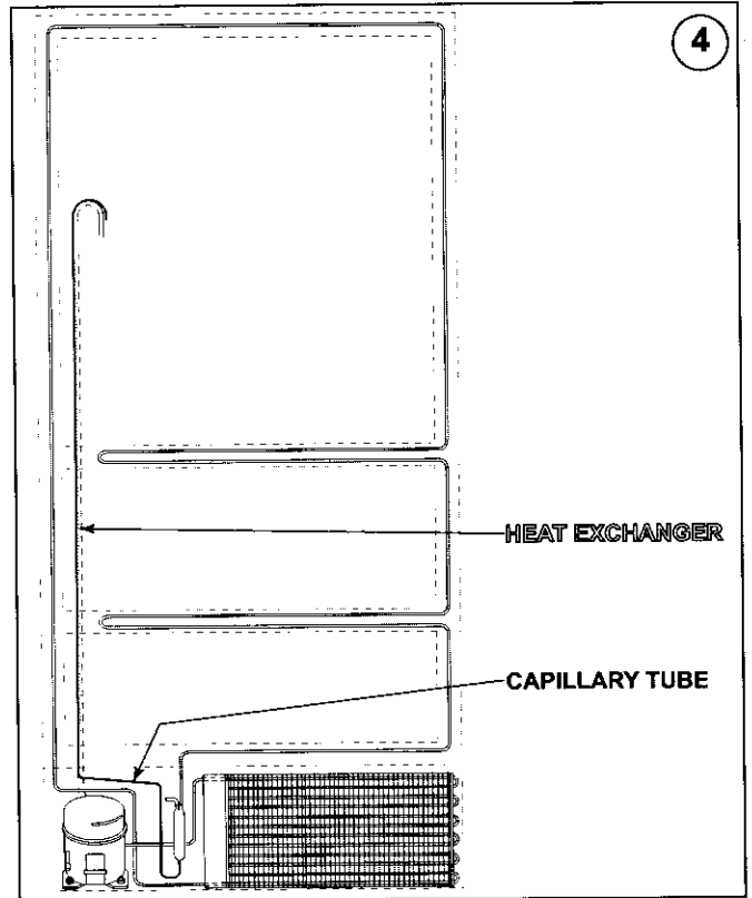
Figure 4-4. Capillary Tube (& Heat Exchanger)
