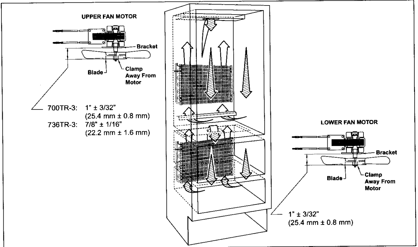
Figure 5-2. 700TR-3 and 736TR-3 Air Flow and Fan Blade Spacing
